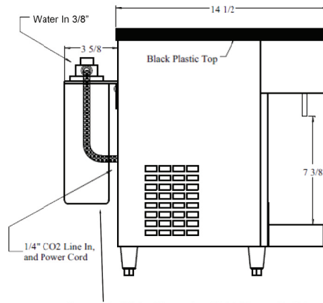
Pre-mounted Water filter system, Quick Change Cartridge.
