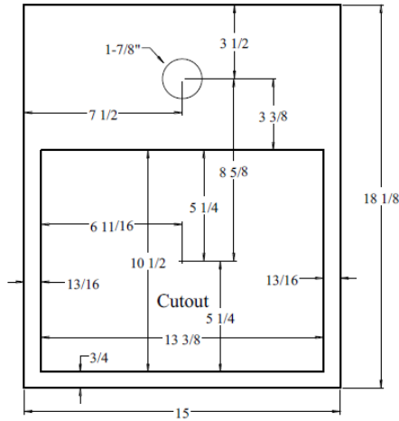
RDP-3-SSQ hole cut and dimensions
