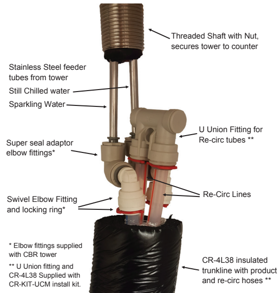
CBR Tower to Trunkline Hook-up
